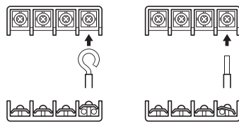
Stripping wire at terminal block
