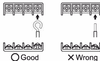
Stripping wire at terminal block
